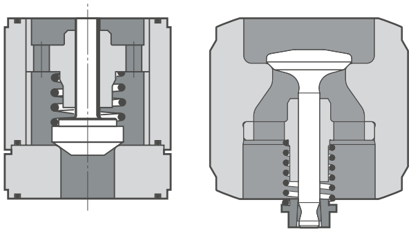
Cone valve
