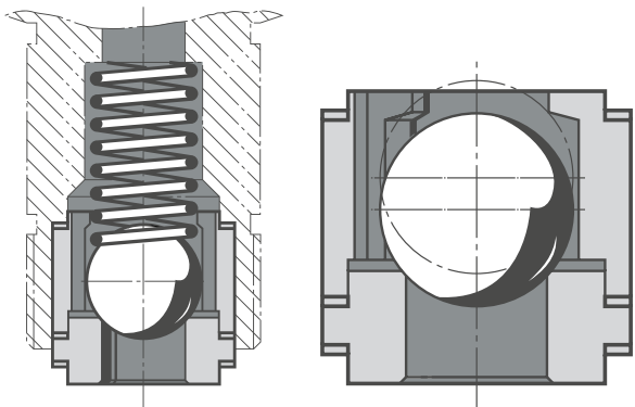
Ball valve
