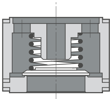
Disc valve
